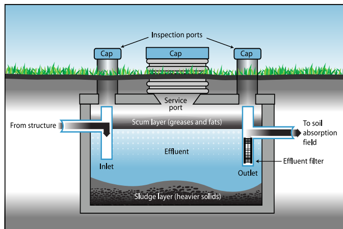
Figure 2. This diagram of a septic tank shows the three layers of waste: scum, effluent, and sludge.
